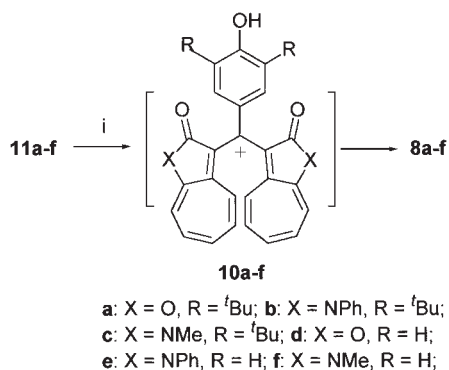
Scheme 3. Reagents and conditions: i, Zn, 3% HCl, AcOH, reflux, 8 h.
