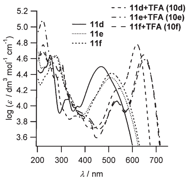
Fig. 3. UV-vis spectra of 11d-f in CH 3 CN and in CH 3 CN and TFA.
