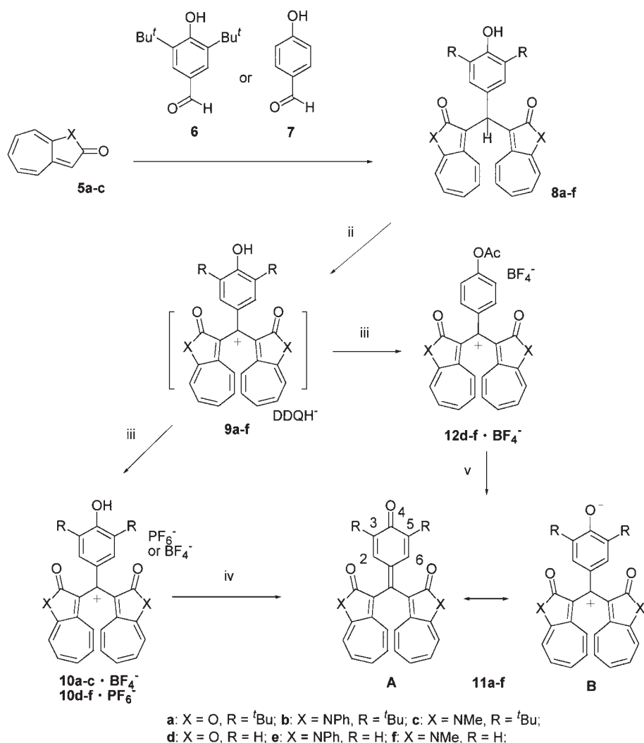
Scheme 1. Reagents and conditions: i, \text{CHCl}_3 –TFA (5:1), reflux, 8 h; ii, DDQ, \text{CH}_2\text{Cl}_2 , rt, 1 h; iii, 60% \text{HPF}_6 or 42% \text{HBF}_4 , \text{Ac}_2\text{O} , 0 °C, 1 h; iv, aq. \text{NaHCO}_3 ; v, \text{K}_2\text{CO}_3 .
