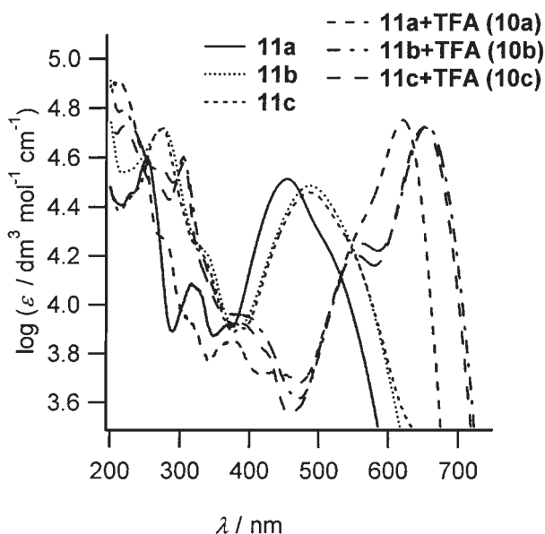
Fig. 2. UV-vis spectra of 11a-c in CH 3 CN and in CH 3 CN and TFA.
